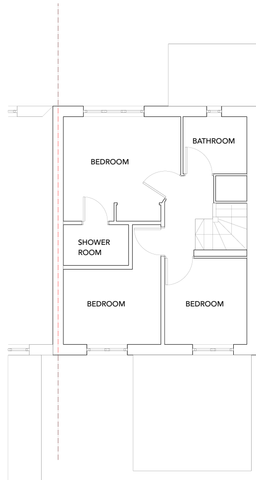
FIRST FLOOR PLAN scale 1:50@A1
