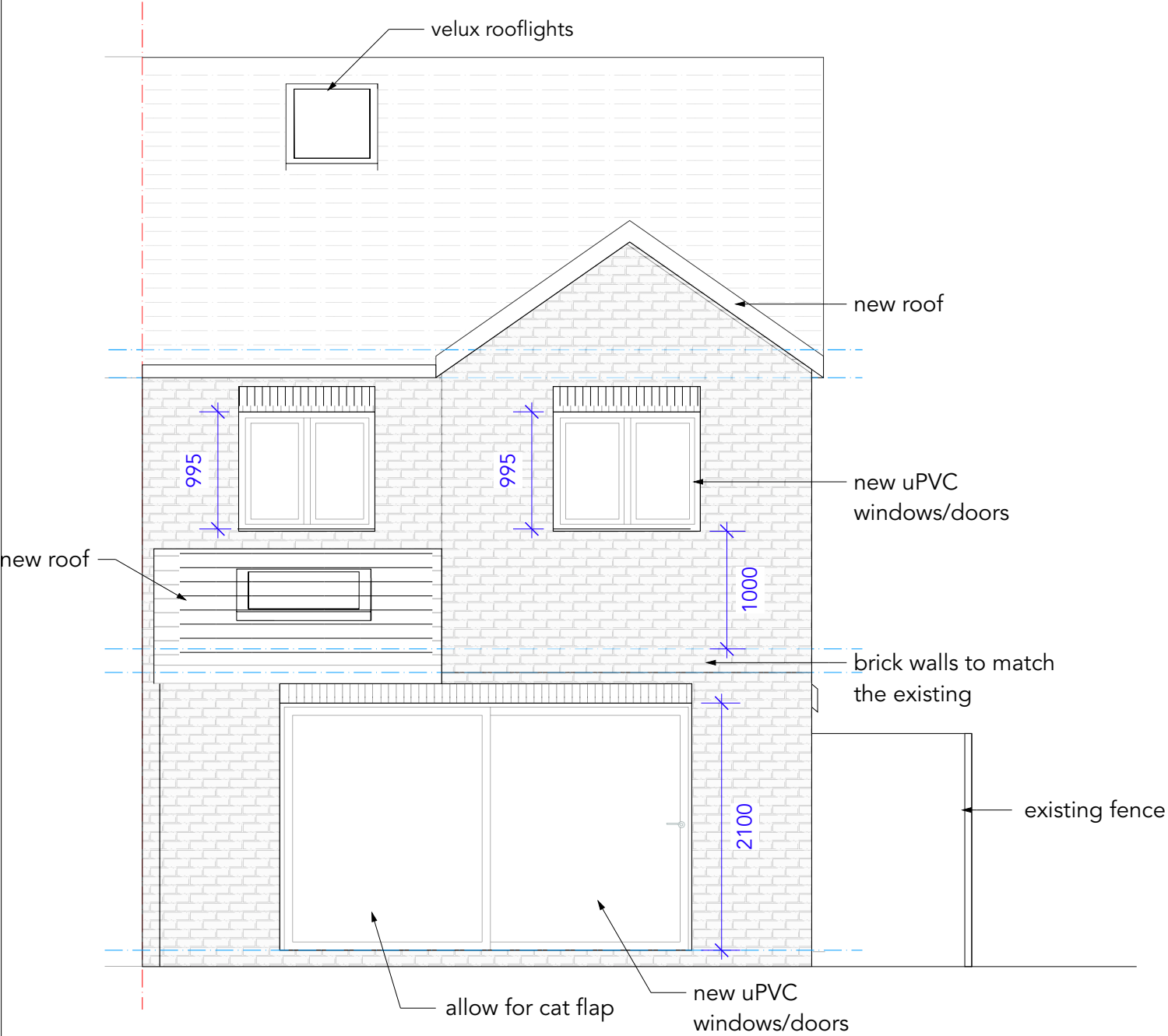
REAR ELEVATION scale 1:50@A1
