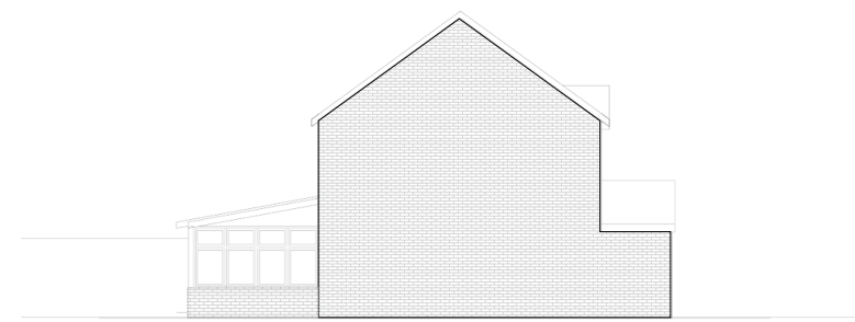
SIDE ELEVATION scale 1:100@A1
